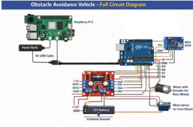
Figure 2: Electric circuit diagram
